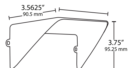
490698 4" Small Shroud
