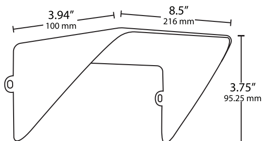
490700 4" Large Shroud
