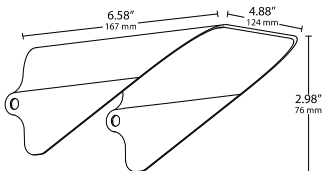
490701 6" Small Shroud
