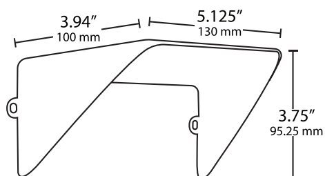
490699 4" Medium Shroud
