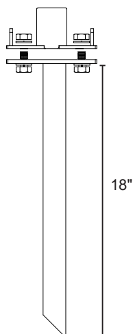
Optional turf stake mount (Kit 489605)
