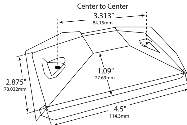
Mounting Plate
