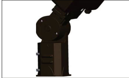
Slipfitter Mount An optional cast aluminum mast arm adaptor secures fixture head to nominal 2" (2-3/8" O.D. pipe size) horizontal steel tenon arm.
